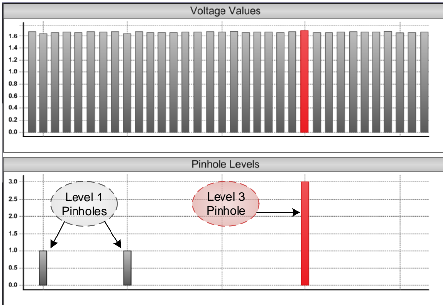
EMOS® Pinhole Detector Results displayed in EMOS® Monitoring
